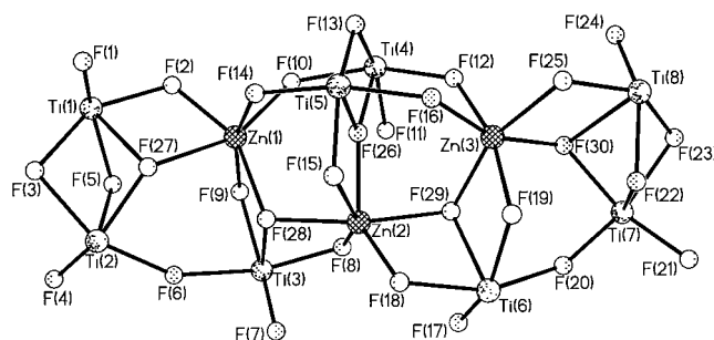
Figure 1. Structure of the inorganic core of 2 in the crystal. For clarity the \text{Cp}^* groups at Ti are omitted. Selected bond lengths [ \text{\AA} ]: \text{Ti-F}_t 1.836* (1.823–1.849), \text{Ti-F}_b 2.034* (1.912–2.317), \text{Zn-F} 2.047* (1.924–2.260), \text{Ti}(1)\text{-F}(2) 1.912, \text{Ti}(1)\text{-F}(3) 2.008, \text{Ti}(1)\text{-F}(5) 1.973, \text{Ti}(1)\text{-F}(27) 2.257, \text{Ti}(2)\text{-F}(27) 2.027(2), \text{Ti}(3)\text{-F}(28) 2.139, \text{Ti}(4)\text{-F}(26) 2.120, \text{Ti}(5)\text{-F}(26) 2.132, \text{Ti}(6)\text{-F}(29) 2.152, \text{Ti}(7)\text{-F}(30) 2.030, \text{Ti}(8)\text{-F}(30) 2.317. The values marked with a * are average values.
